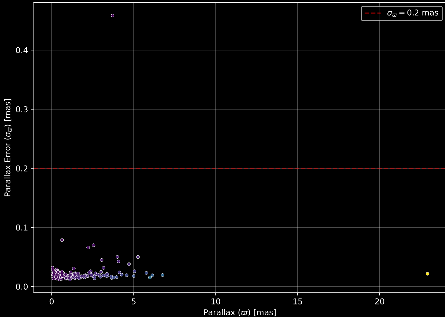
APOGEE DR17 Field: [000+45] Parallax Quality (n= 177)
