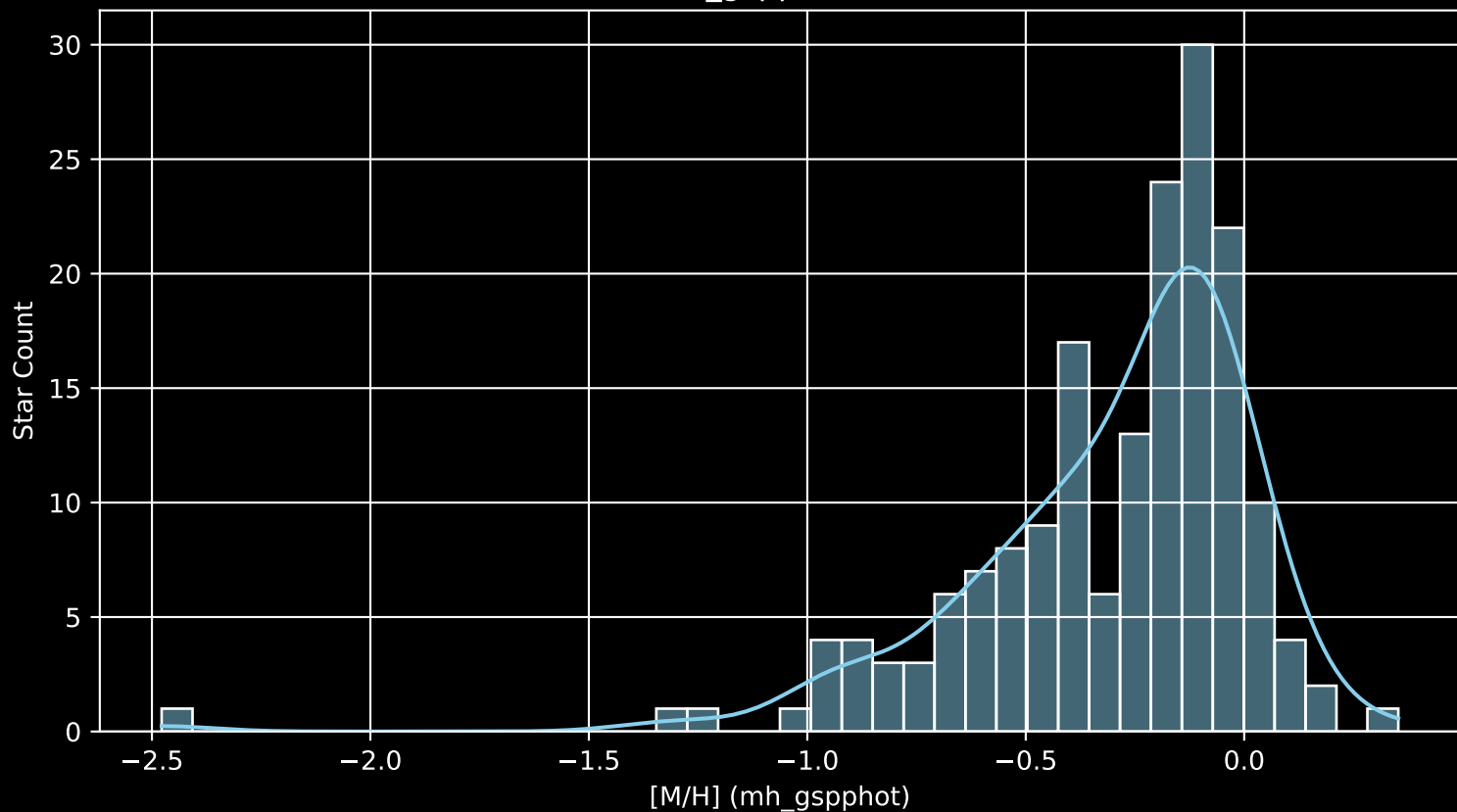
APOGEE DR17 Field: [000+45 [M/H] (mh_gspphot) (n= 177)
