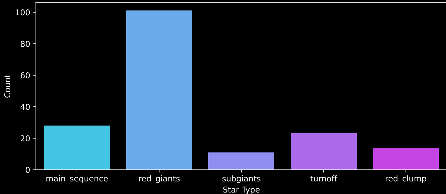
APOGEE DR17 Field: [000+45] Count plot of Star Type
