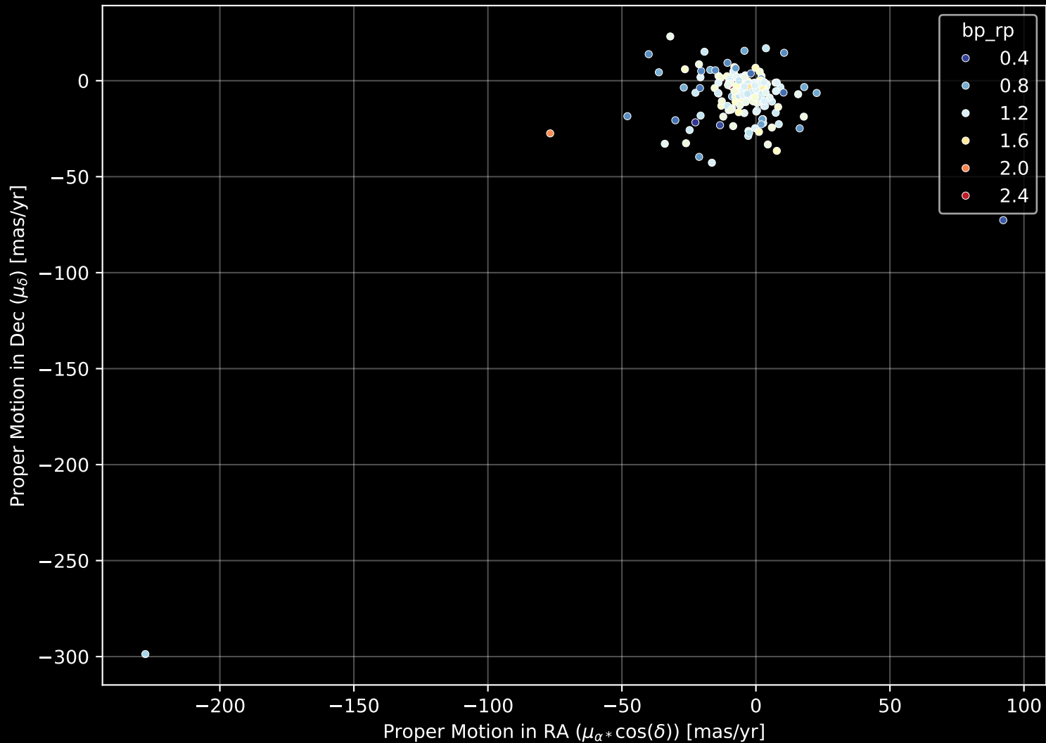
APOGEE DR17 Field: [000+45] Proper Motion Diagram (n= 177)
