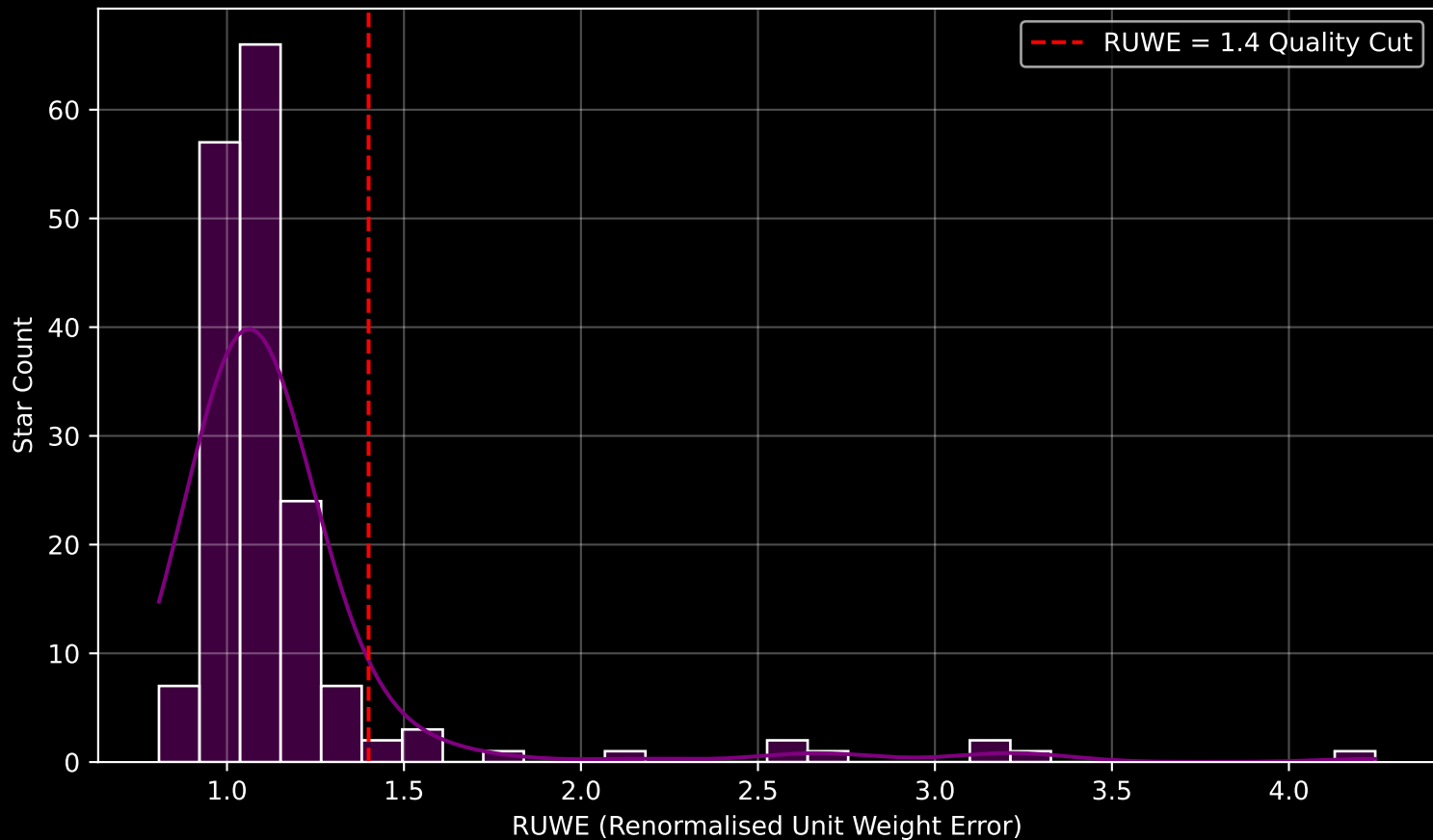
GAPOGEE DR17 Field [000+45] RUWE Distribution (n= 175)
